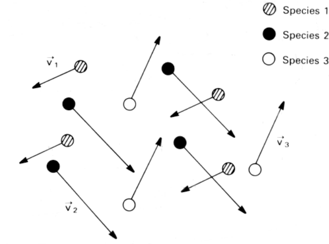
Figure 11.3 Molecules of different species in a mixture moving with different average velocities. The velocity \bar{v}_i is the average over all molecules of species i .
